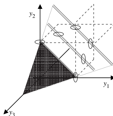
Figure 7. State-space analysis of the LCA model for three alternatives. The grey triangle indicates the attracting plane and dotted lines indicate the intersection of the attracting plane with the y_1 y_3 plane and the y_2 y_3 plane. The thick grey line symbolizes the attracting line in the y_1 y_2 plane; the double grey lines show sample positions of the attracting line in the y_1 y_2 plane for two negative values of y_3 . The two planes surrounded by dashed lines indicate positions of the decision thresholds for alternatives 1 and 2. The ellipses indicate the intersections of the attracting lines in the y_1 y_2 plane with the decision thresholds.
