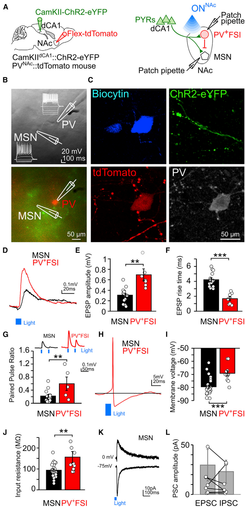
Figure 6. dCA1 Axons Drive Both MSN and PV + FSI Postsynaptic Responses and Exert Feedforward Inhibition on dCA1-Connected MSNs
